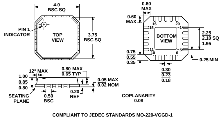
Figure 40. 20-Lead Lead Frame Chip Scale Package [LFCSP] (CP-20-1) Dimensions shown in millimeters
