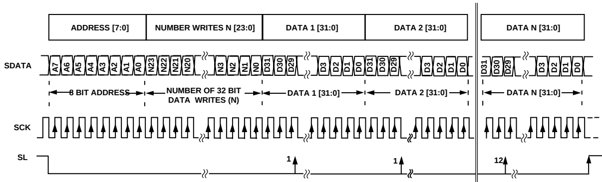
Figure 11. System and Mode Register Writes
