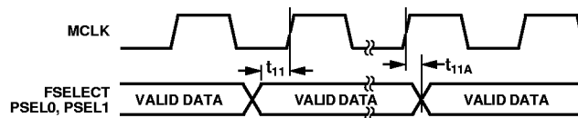
Figure 4. Control Timing
