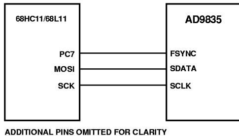
Figure 25. 68HC11/68L11-to-AD9835 Interface
