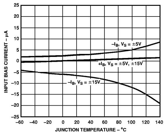
Figure 9. Input Bias Current vs. Junction Temperature
