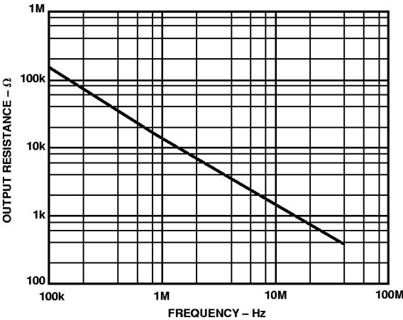
Figure 15. Output Resistance vs. Frequency, Disabled State
