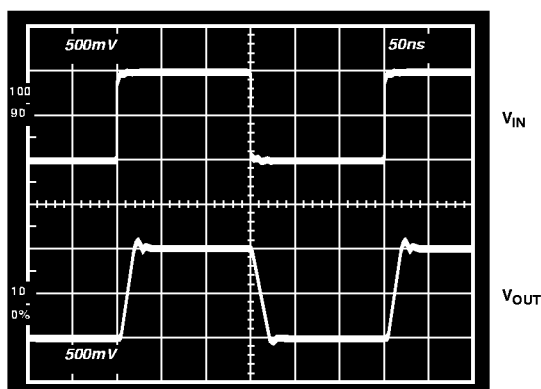
Figure 28. Large Signal Pulse Response, Gain = +10, ( R_F = 357\ \Omega , R_L = 500\ \Omega , V_S = \pm 15\ \text{V} )
