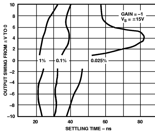
Figure 21. Output Swing and Error vs. Settling Time
