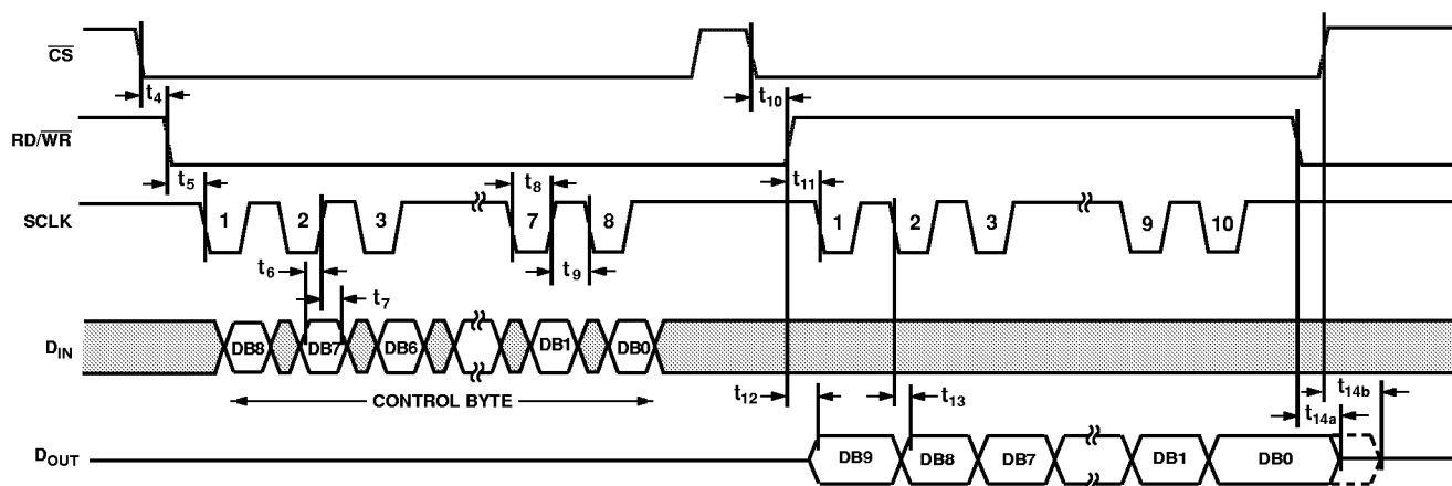
Figure 20. AD7817 Serial Interface Timing Diagram
