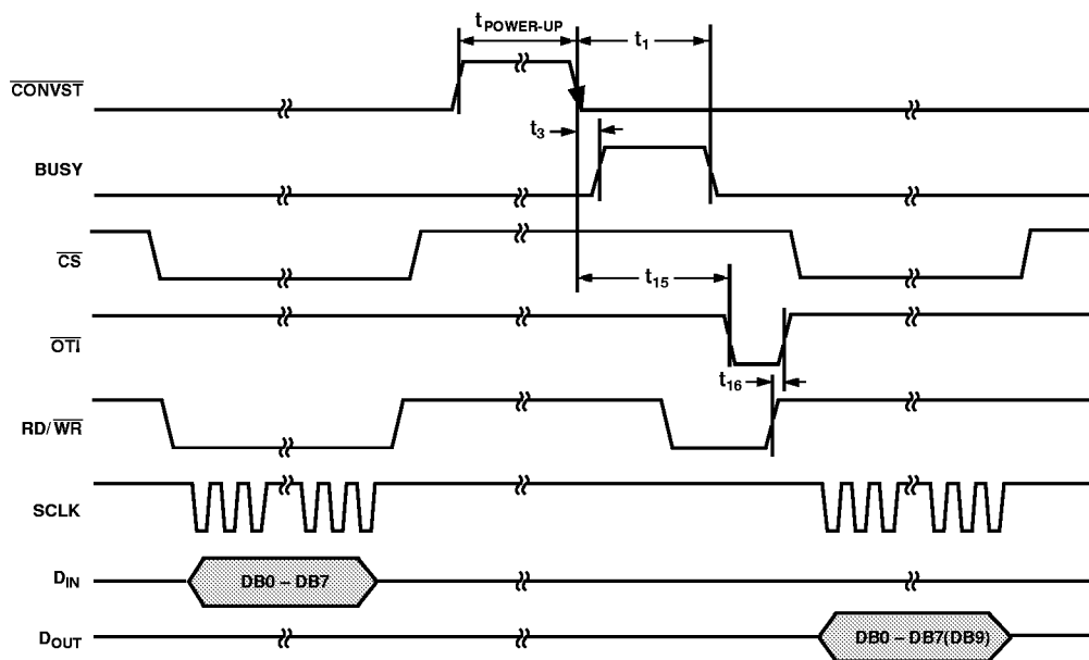
Figure 17. Mode 2 Operation
