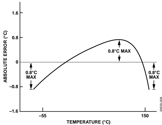
Figure 12. Nonlinearity
