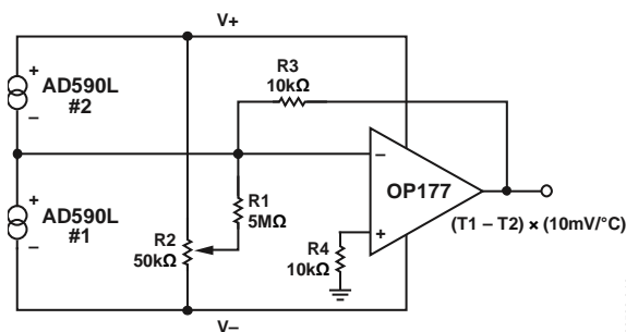
Figure 19. Differential Measurements
