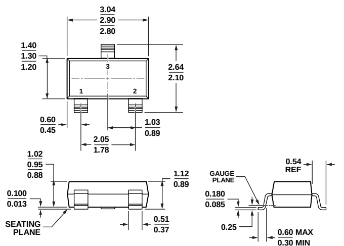
Figure 27. 3-Lead Small Outline Transistor Package [SOT-23-3] (RT-3)
