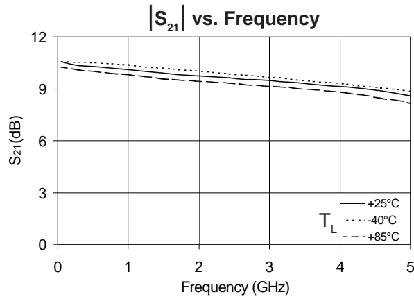
Typical RF Performance Over Temperature (Bias: V_D=2.2V , I_D=20\text{ mA} (Typ.))
