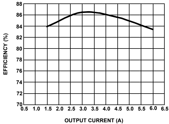
FIGURE 8. MEASURED EFFICIENCY V_{IN} = 12\text{V} , V_{OUT} = 3.3\text{V}
