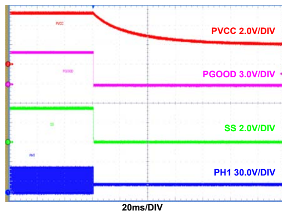
FIGURE 12. EN SHUTDOWN, PVCC/PGOOD/SS FALL, I_{OUT} = 0A
