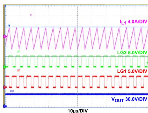
FIGURE 14. CCM MODE (DE/PHDRP = GND), PHASE 1 INDUCTOR RIPPLE CURRENT, I_{OUT} = 0A
