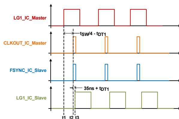
FIGURE 56. TIMING DIAGRAM OF CLKOUT vs LG1 AND FSYNC vs LG1 (CLKOUT_MASTER CONNECTED TO FSYNC_SLAVE)
