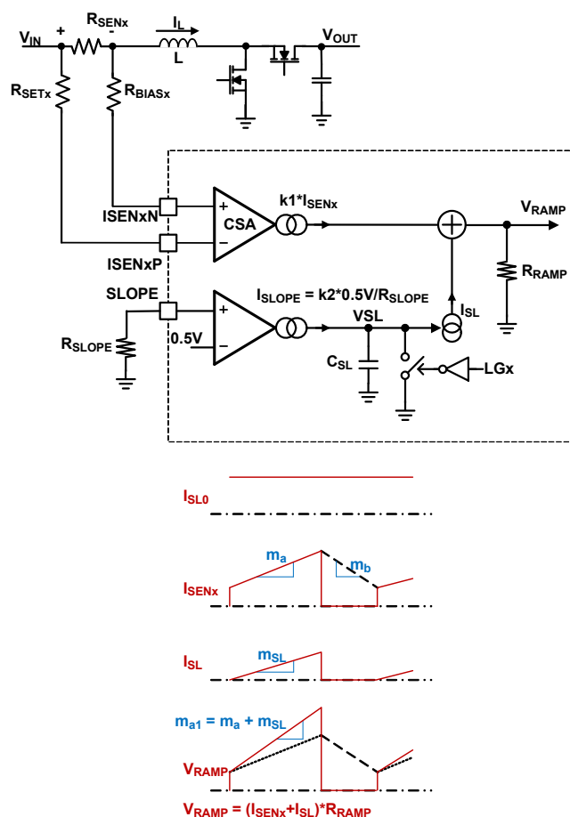
FIGURE 61. SLOPE COMPENSATION BLOCK DIAGRAM
