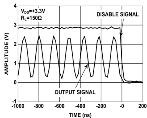
FIGURE 16. DISABLE TIME
