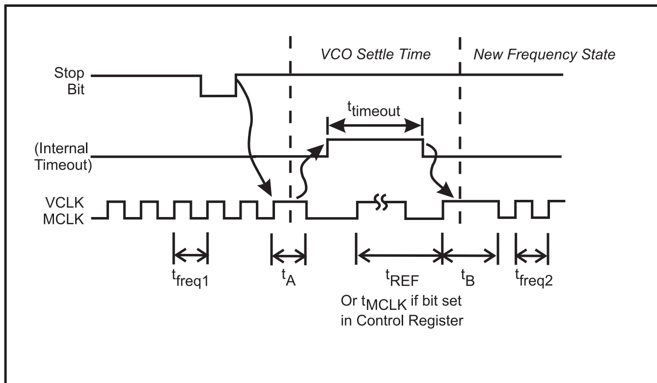
MCLK and Active VCLK Register Programming Timing
