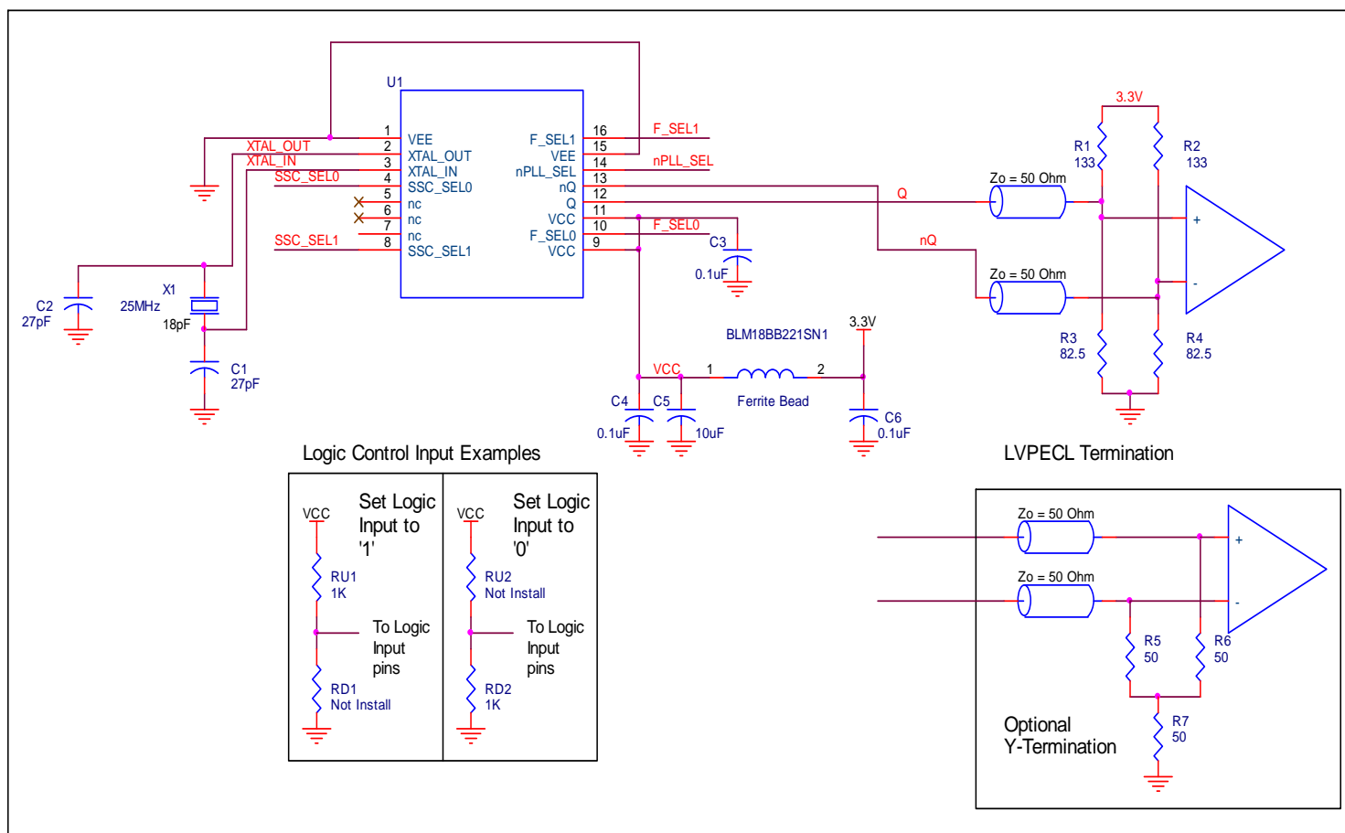
Figure 3. 843441 Schematic Example
