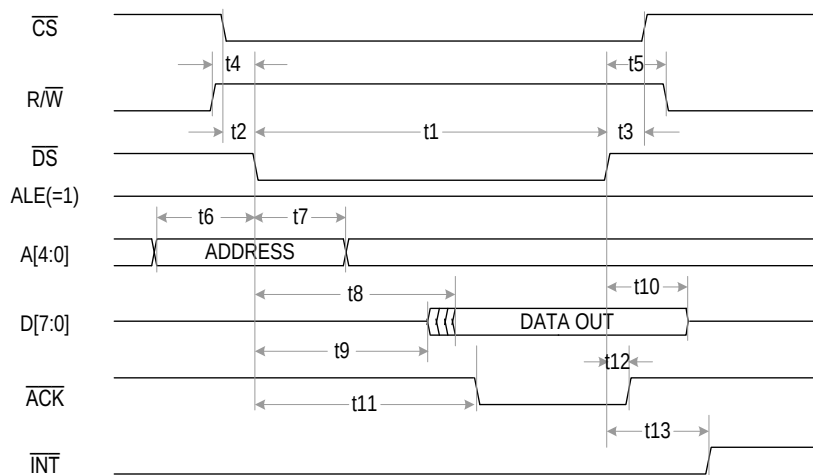
Figure-33 Non-Multiplexed Motorola Mode Read Timing
