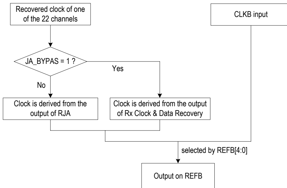
Figure-39 REFB Output Options in Normal Operation
