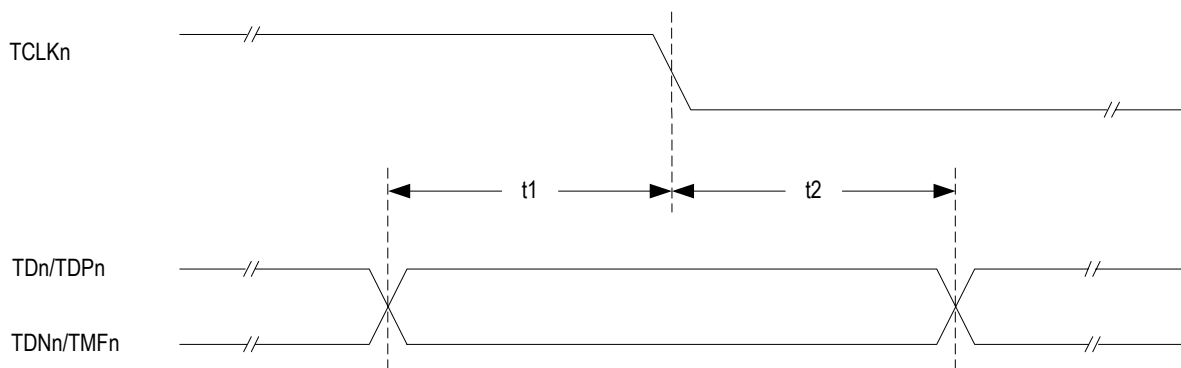
Figure-49 Transmit Clock Timing Diagram
