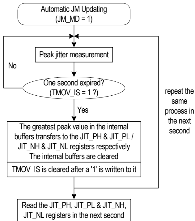
Figure-36 Automatic JM Updating
