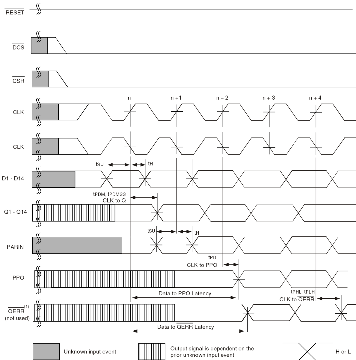
Timing Diagram for the First IDT74SSTUAE32866A (1:2 Register-A Configuration) Device Used in a Pair; C0 = 0, C1 = 1, \overline{\text{RESET}} Held HIGH
