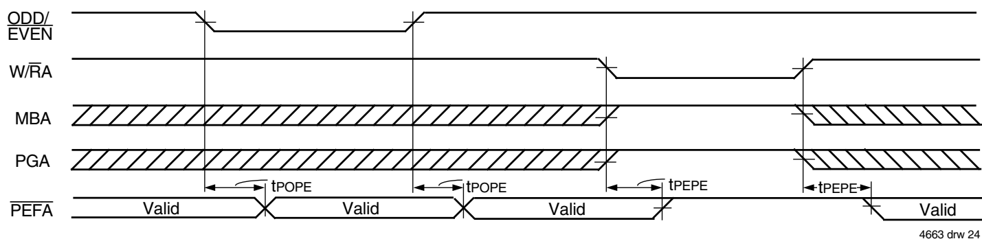
Figure 24. \text{ODD}/\overline{\text{EVEN}} , \overline{\text{W}}/\overline{\text{RA}} , \overline{\text{MBA}} , and \overline{\text{PGA}} to \overline{\text{PEFA}} Timing
