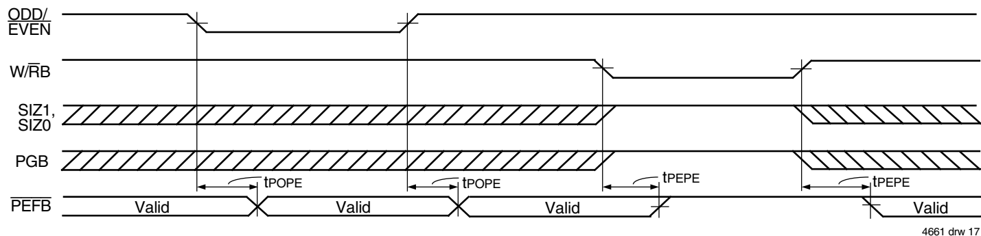
Figure 17. \text{ODD}/\overline{\text{EVEN}} , \overline{\text{W}}/\overline{\text{RB}} , SIZ1, SIZ0, and PGB to \overline{\text{PEFB}} Timing
