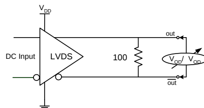
V_{OD} SETUP
