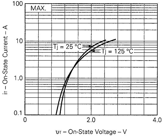
Fig. 1 i_r - v_T CHARACTERISTIC
