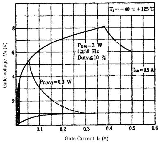
Figure 3. Gate Rating
