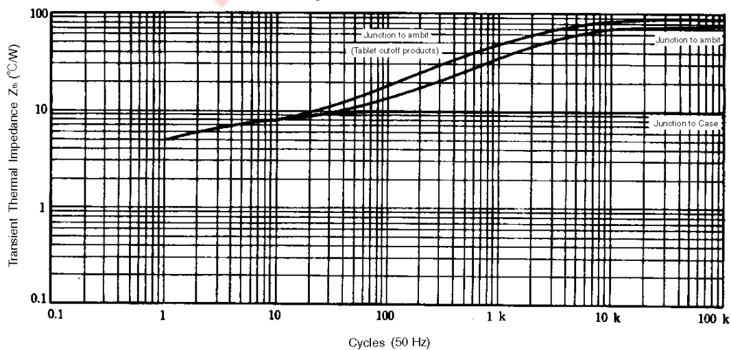
Figure 13. Z_{th} Characteristics
