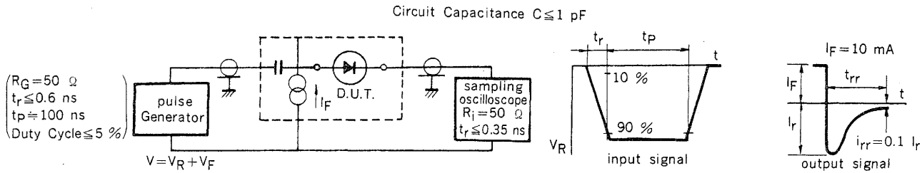
Test circuit I_F = 10 mA, V_R = 6.0 V
