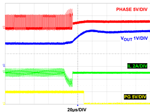
FIGURE 46. OVERVOLTAGE PROTECTION
