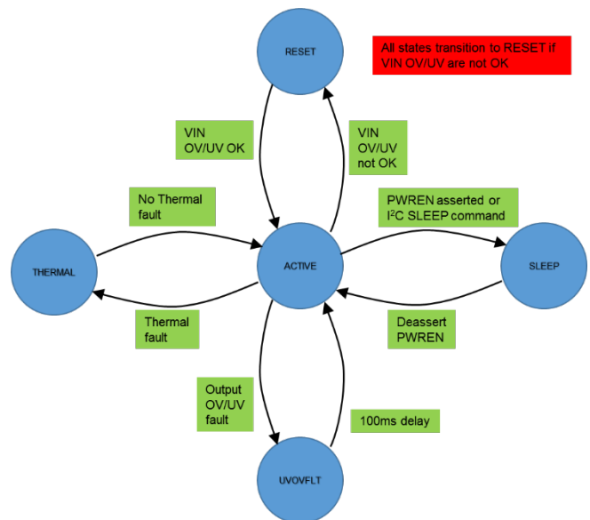
Figure 4. State Machine
