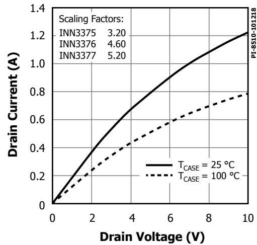
Figure 49. Output Characteristics.
