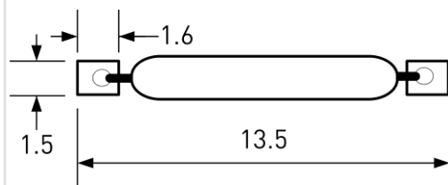
Pad sizes
