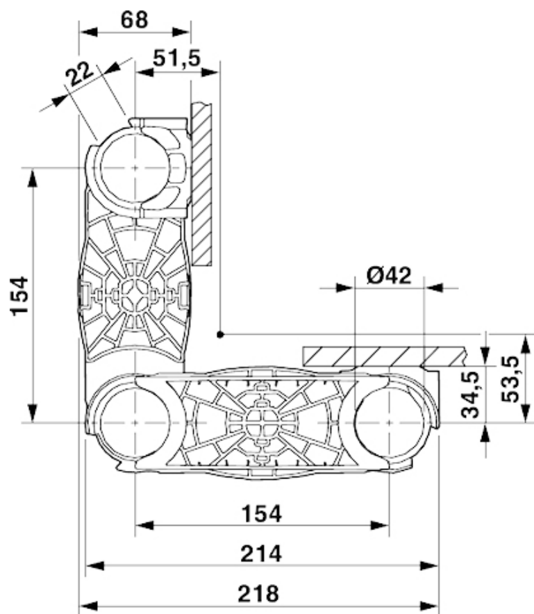
Dimensional drawing
