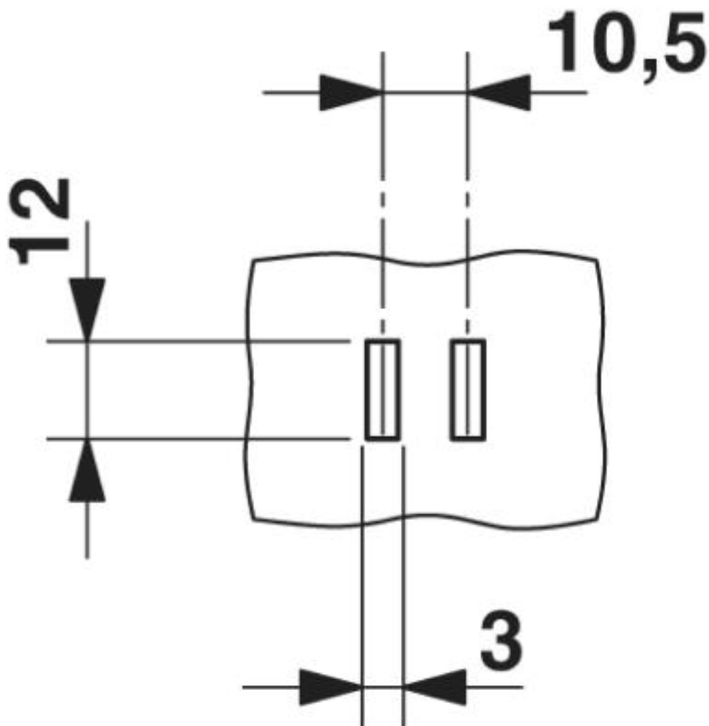
Dimensional drawing
