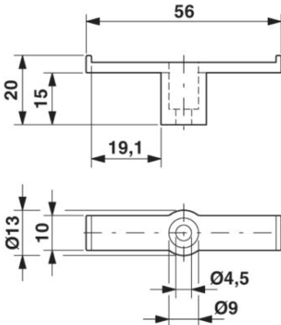
Dimensional drawing
