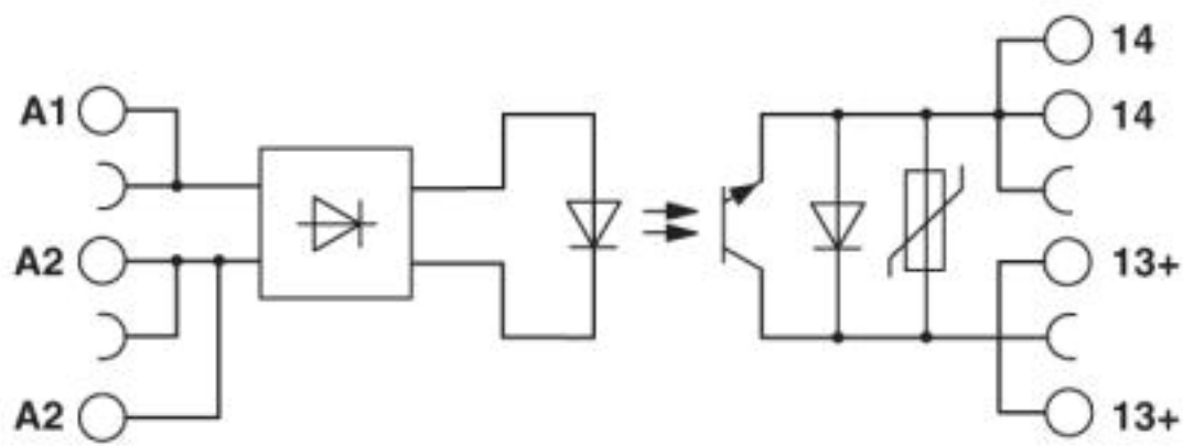
Circuit diagram
