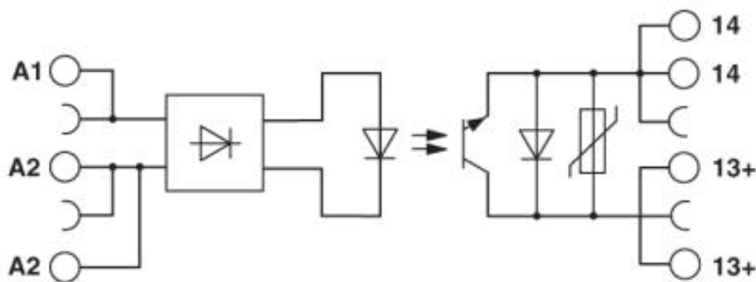
Circuit diagram
