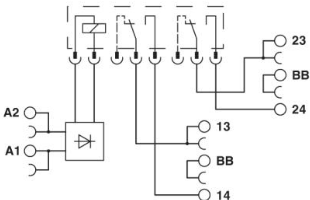
Circuit diagram
