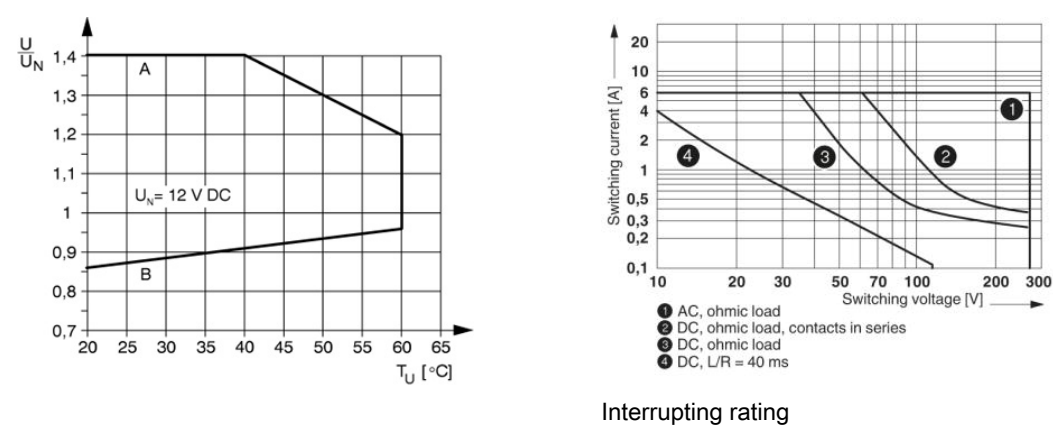
Interrupting rating
