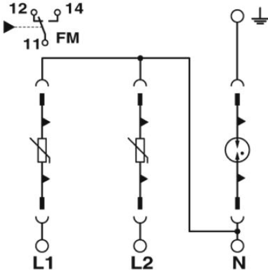
Circuit diagram
