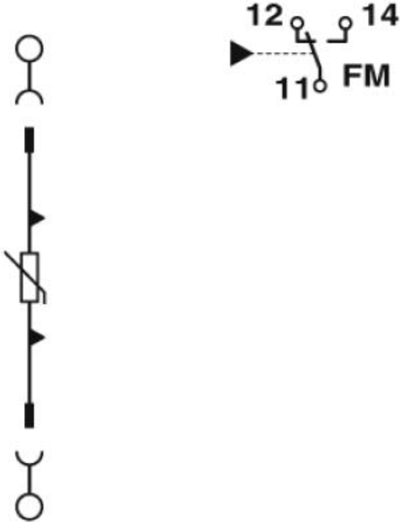
Circuit diagram
