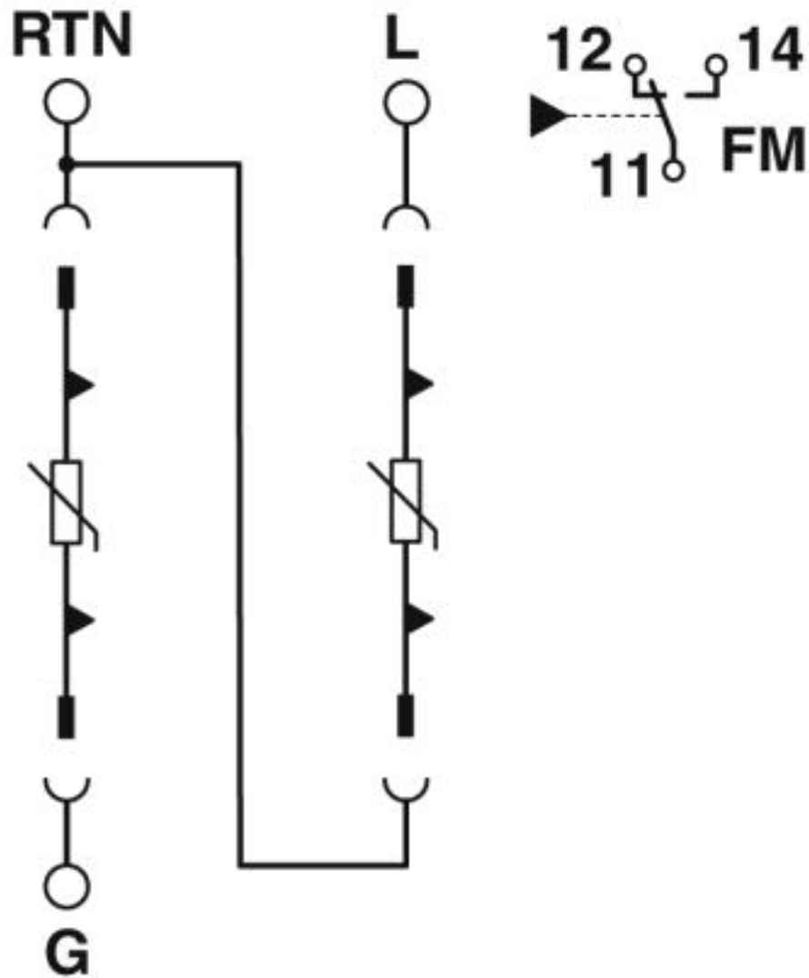
Circuit diagram
