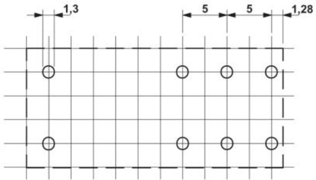
Drilling diagram
