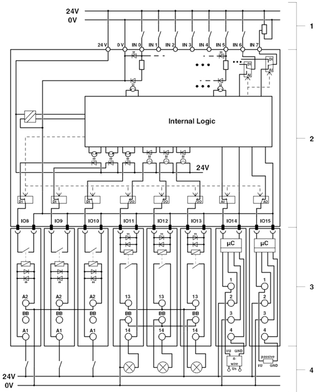
Circuit diagram
