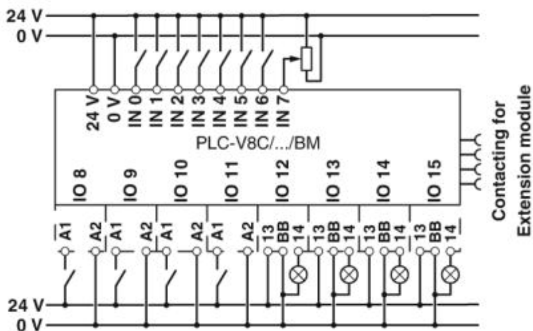
Connection diagram
