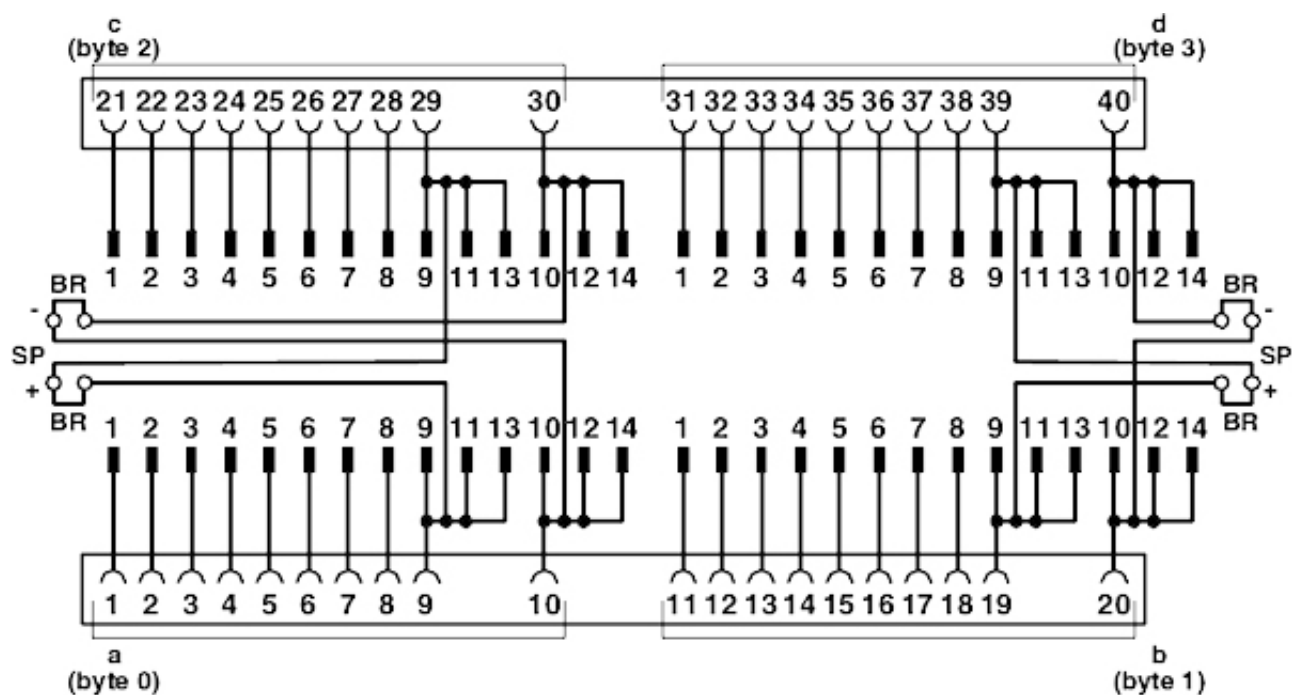
Circuit diagram
