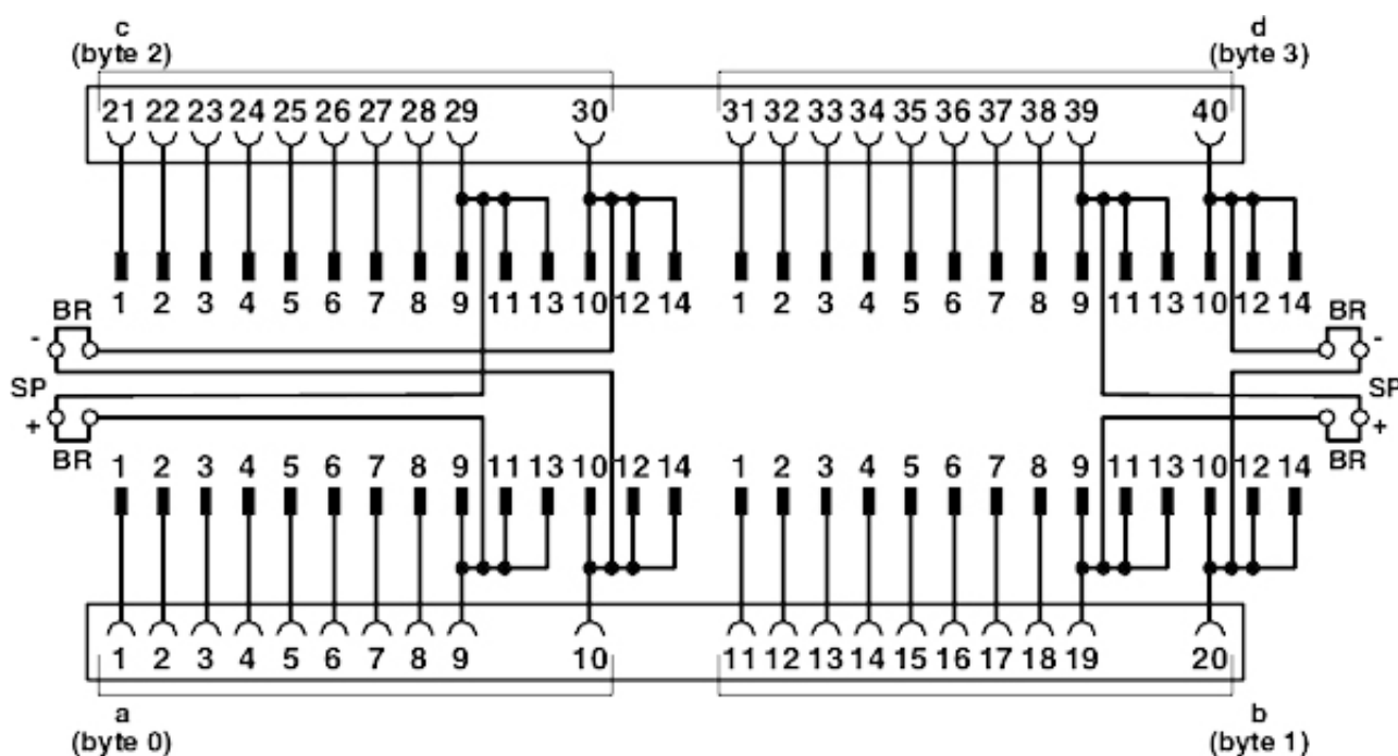
Circuit diagram
