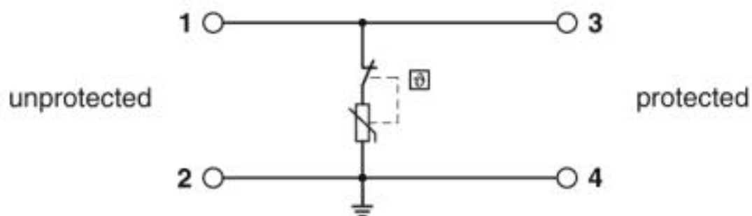
Circuit diagram
