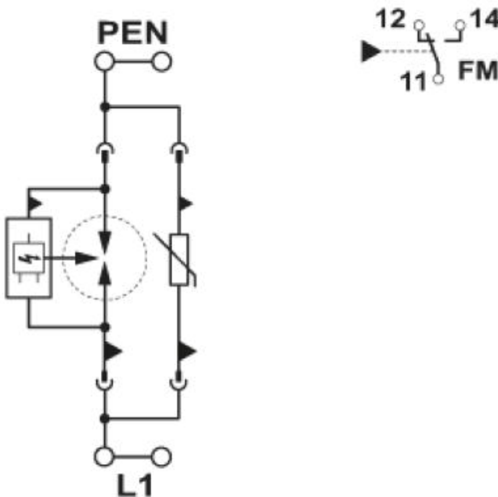
Circuit diagram
