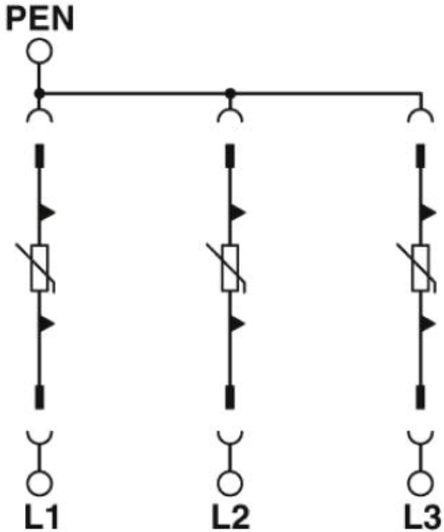
Circuit diagram
