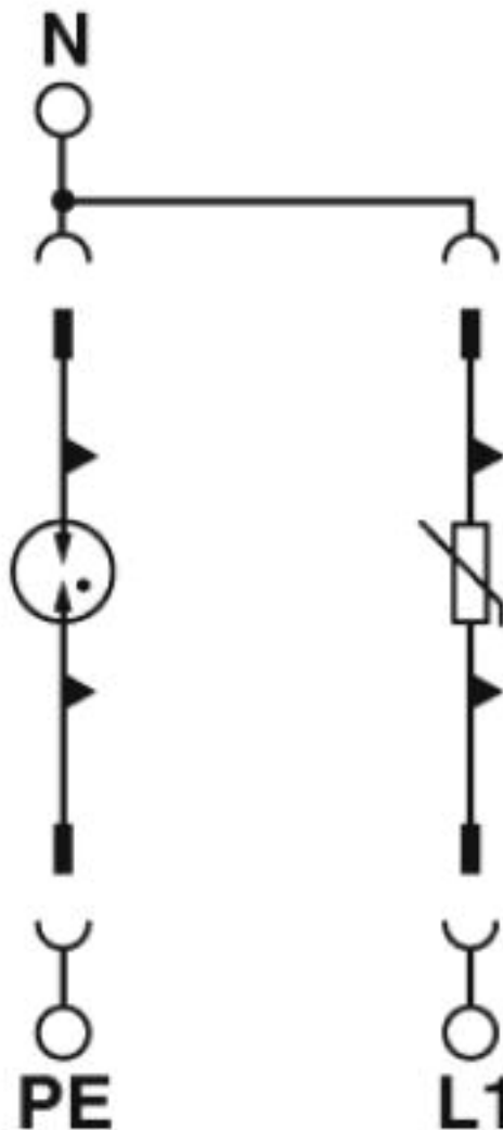
Circuit diagram
