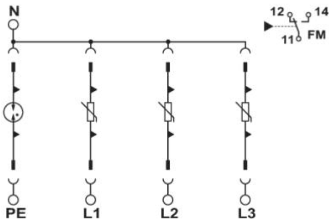
Circuit diagram
