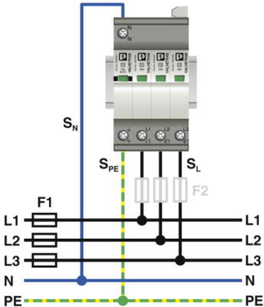
Application drawing
