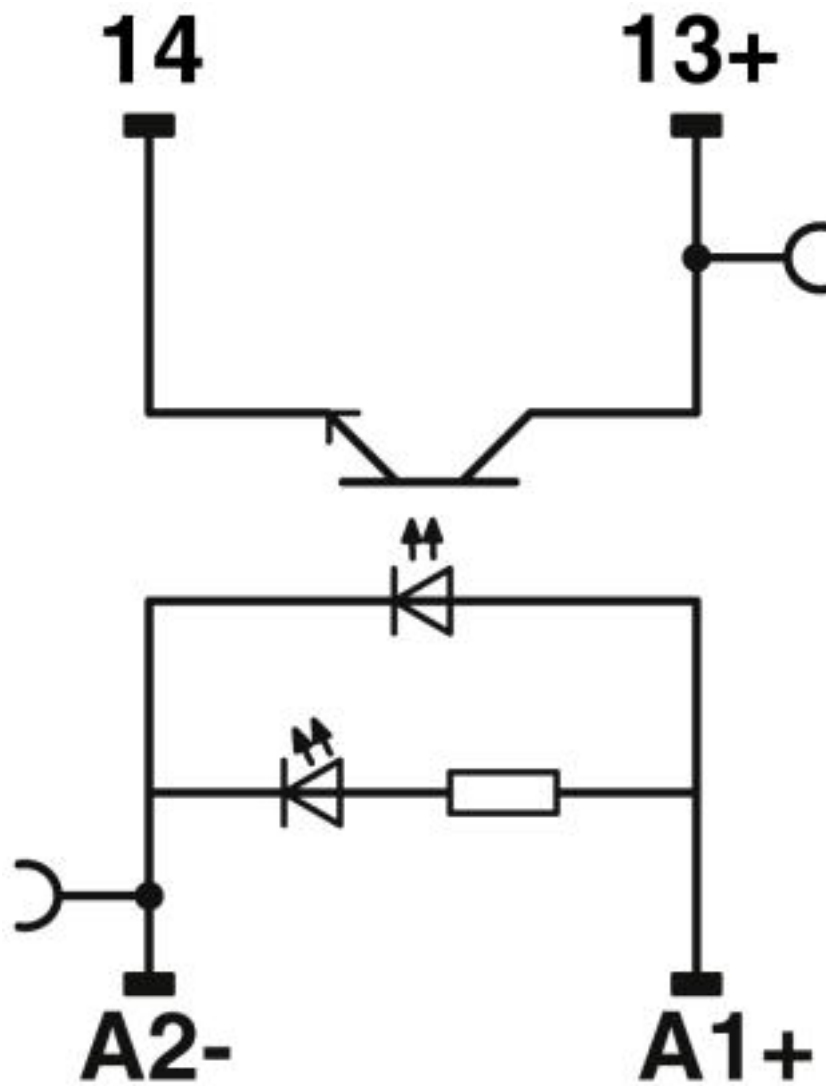
Circuit diagram
