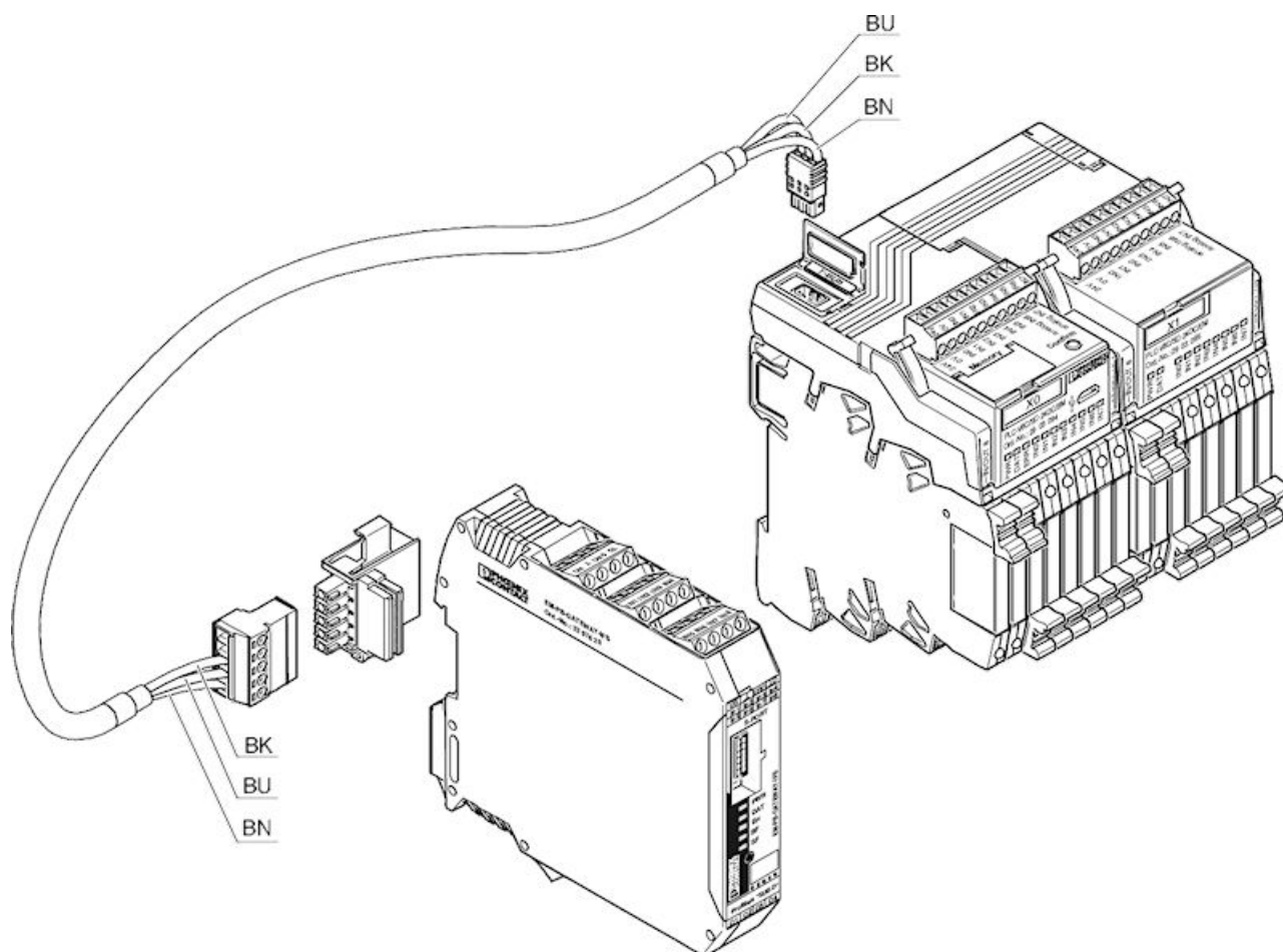
Schematic diagram
