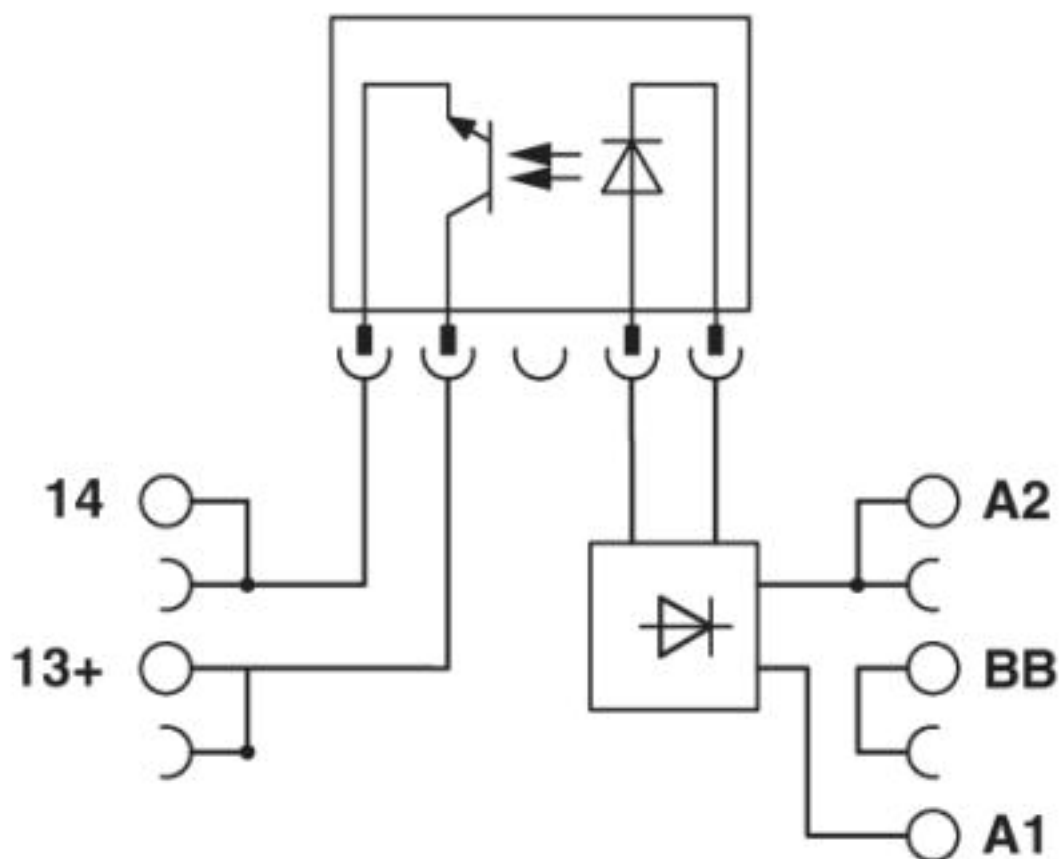
Circuit diagram
