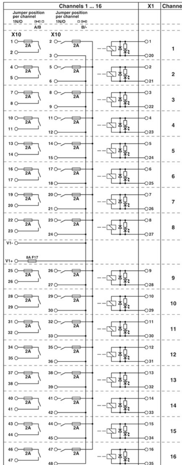
Circuit diagram
